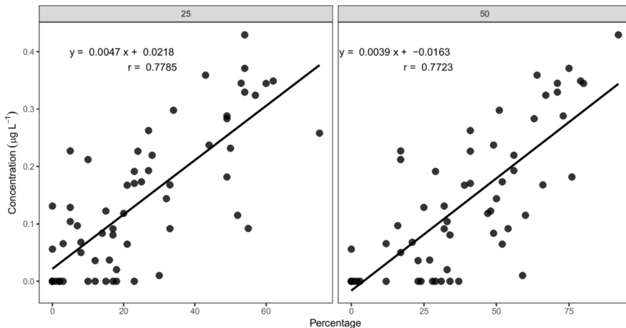
Figure 14: Linear regression between percentage of groundwater samples younger than 25 (left) or 50 (right) years and TFA concentrations. For instance, if the percentage of groundwater younger than 25 years is 60%, a concentration of 0.3 \mu\text{g/L} of TFA can be expected in groundwater.
