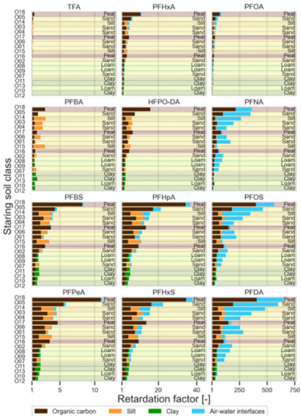
Figure 5: Retardation of 12 PFAS compounds, from TFA to PFDA, for 18 soil types in The Netherlands, at the average saturation for an infiltration factor q = 300 \text{ mm/yr} (van den Berg, 2023). Each bar shows the retardation factor in a given soil, with colors representing the cause of retardation. The plots for the different PFAS are sorted in columns by the mean retardation of that PFAS (note the different horizontal scales for each column), and the soils within the plot are sorted by the mean retardation for PFOA. The colors of the background represent the soil class, which is labelled on the right.
