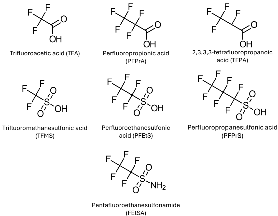
Figure 1. Chemical structure of TFA and other ultrashort-chain PFAS.
