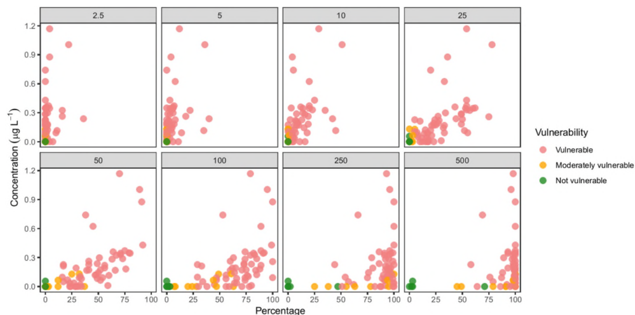
Figure 13: Correlations between the percentage of groundwater of a specific age range (from 2.5 to 500 years old) and its TFA concentration.
