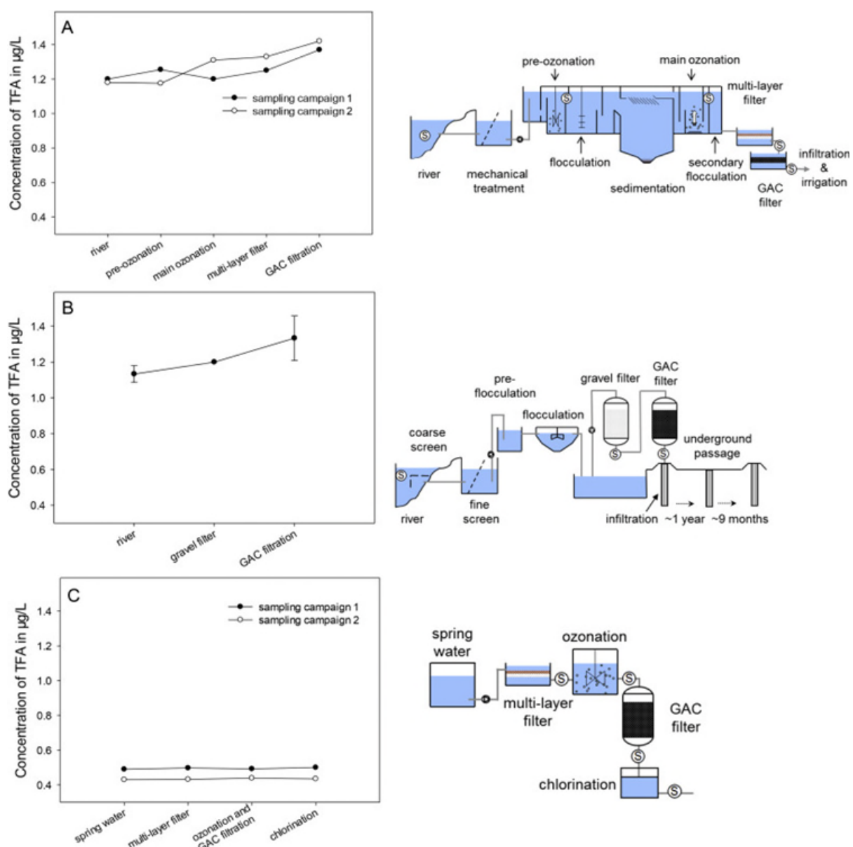
Figure 6: TFA concentrations along the treatment train of three waterworks and schemes of the investigated treatment plants (Scheurer et al., 2017).
