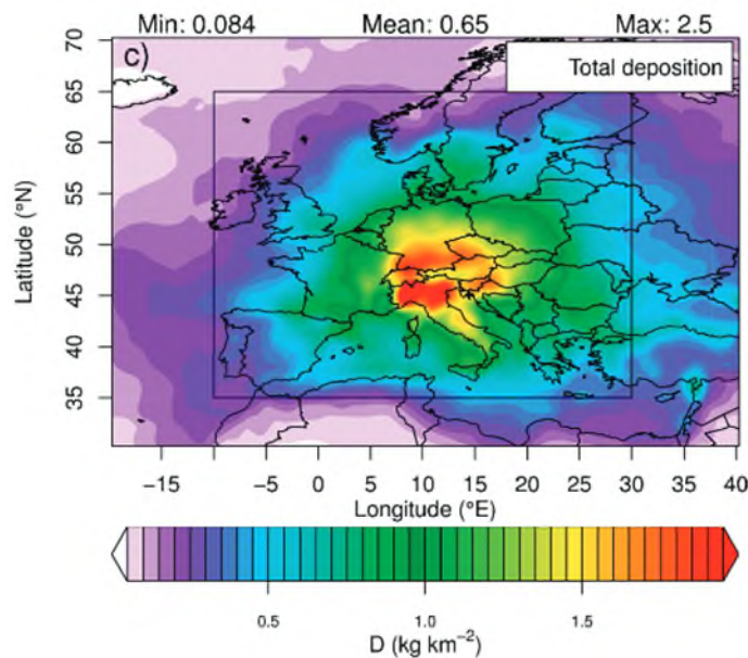
Figure 3. Simulated TFA annual deposition rates (dry and wet) (Henne et al., 2012).
